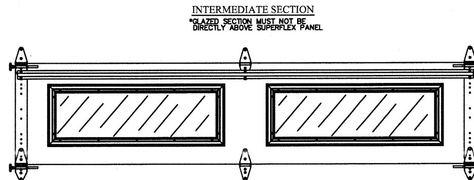
OPTIONAL GLAZED SECTION W/LONG PANEL IMPACT WINDOWS N.T.S.
