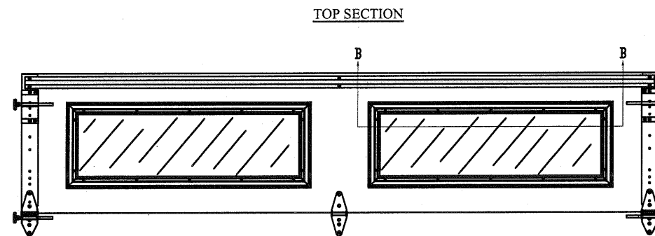
OPTIONAL GLAZED SECTION W/LONG PANEL IMPACT WINDOWS N.T.S.
